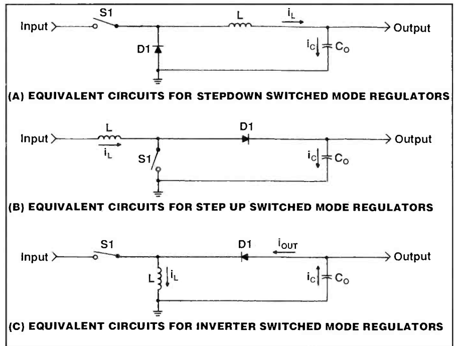
Figures 8. A, B, and C illustrate the operation of a step-down switched-mode regulator, a step-up switched-mode regulator, and an inverting switched-mode regulator through equivalent circuits.
