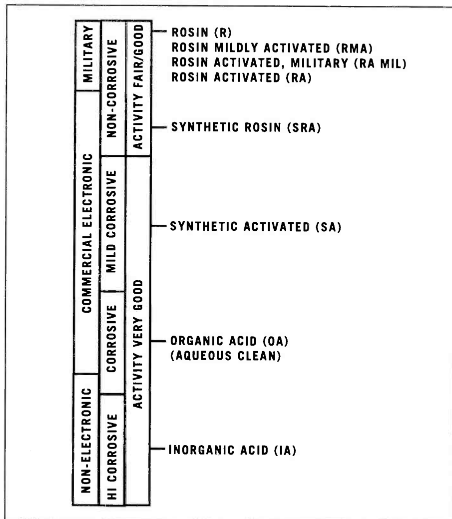
Figure 4. From the standpoint of soldering iron tip plating corrosion, the less active the soldering flux, the lower the chance that the plating will be eaten away. Shown here is an activity ranking of various flux types. RMA fluxes have proven to yield the best tip life.
