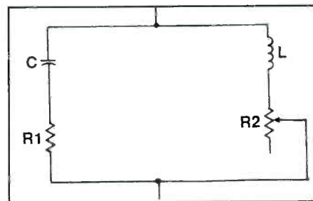
Figure 2. Can you adjust the frequency of this circuit by varying the resistance of R_2 ?
