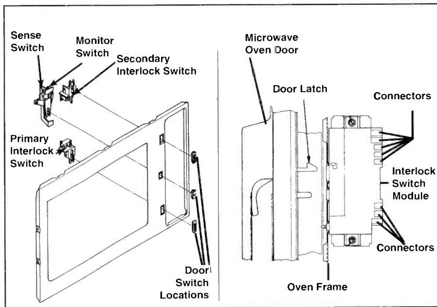
Figure 4. Drawing A shows the door switch assembly. B shows the interlock switch module.
