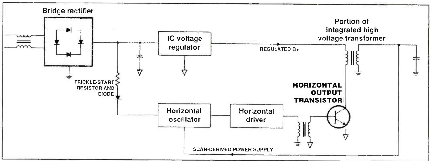
Figure 4. The trickle-start system shown here is one method for starting the oscillator in a scan-derived power supply.
