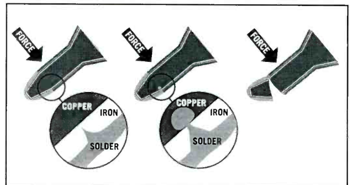
Figure 2. If the iron plating on the soldering iron tip cracks, once the copper core is exposed, solder will quickly dissolve some of the copper away, hollowing out the tip.
