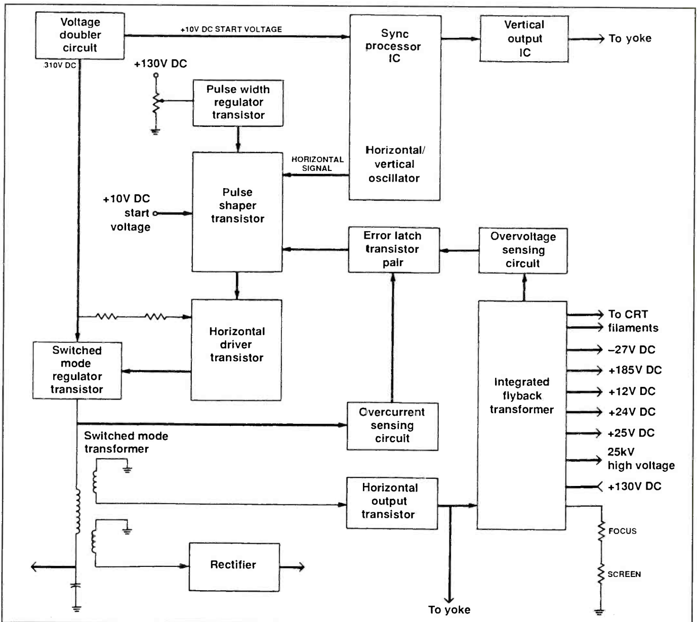
Figure 5. This block diagram of a color television power supply system illustrates how a system operating at the horizontal sweep frequency can establish the low and high voltages needed for the entire receiver, the tuner and tuner control system, I-F signal processing systems, video and chrominance processing systems, audio systems, vertical deflection systems, the CRT anode and focus voltages, and the CRT screen, or G2, control.
